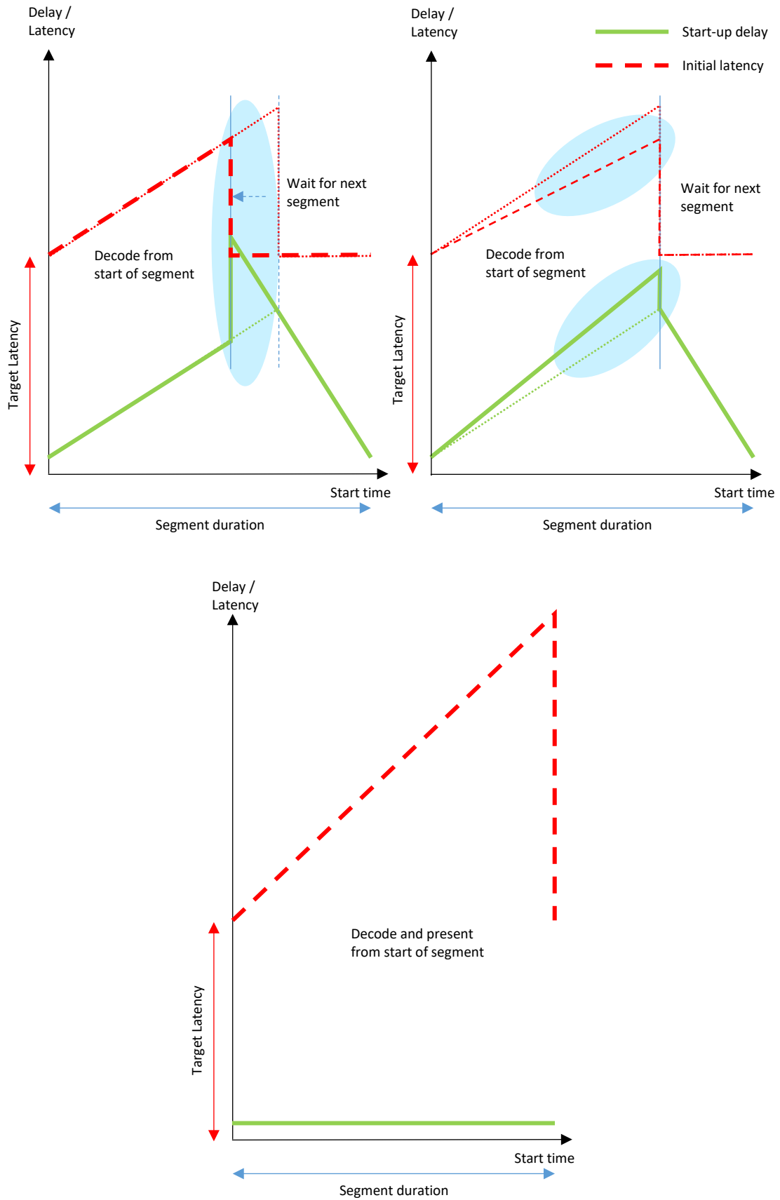
Figure 5: Start-up delay and latency trade-offs
