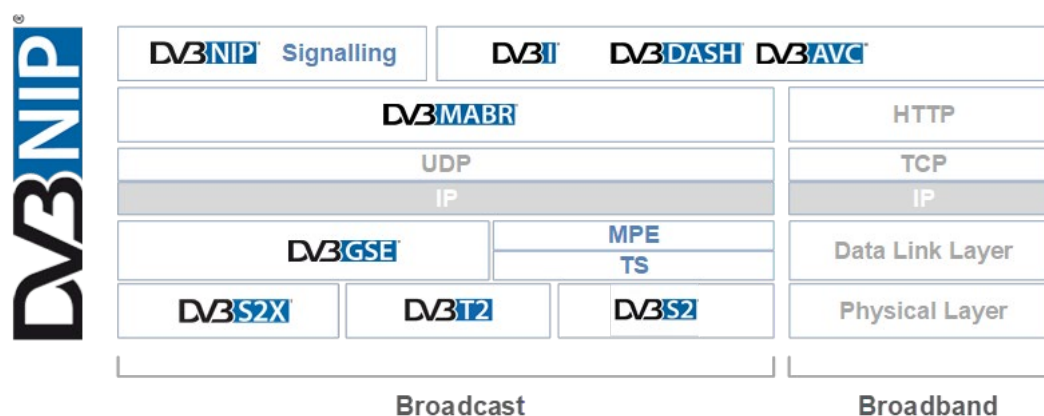
Figure 5.2.1-1: DVB-NIP protocol stack
