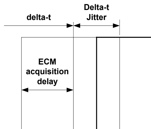
Figure 6: Delta-t Jitter
