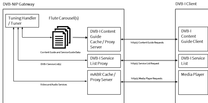
Figure D 5.3.2 Client-Gateway Interaction for the NIP Content and Service Guide
