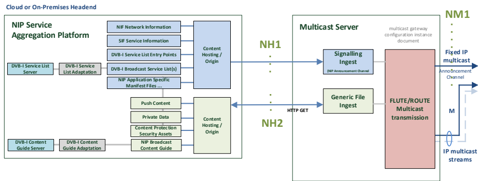
Figure 9.5.5-1: Logic for building the NIP Content Guide documents for Broadcast
