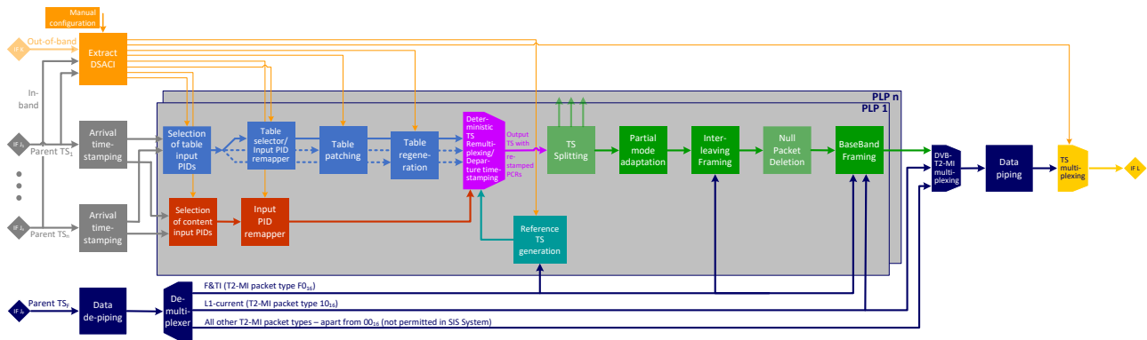
Figure 5: DSA processing (DVB-T2 case)
