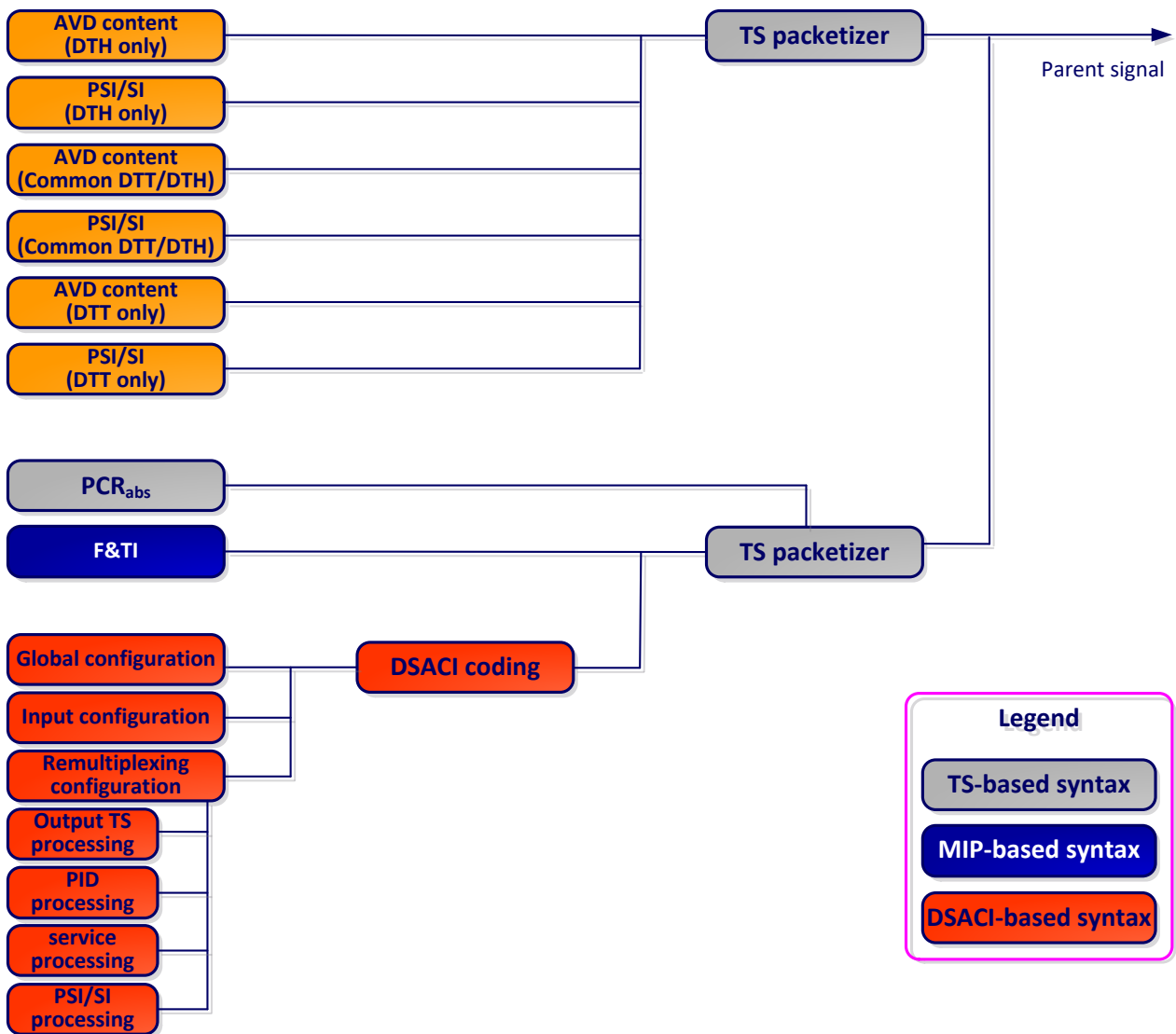
Figure 4: Parent Signal composition illustrating metadata and Audio/Video/Data content, DVB-T case
