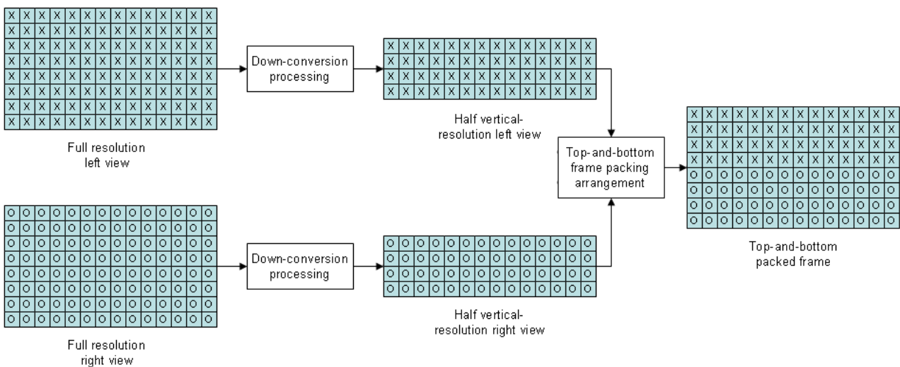
Figure 10 Top-and-Bottom video frame composition
